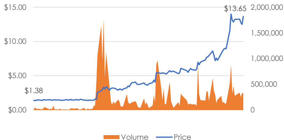
ZDGE Stock Price and Volume
